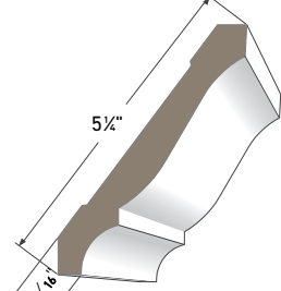
6" Crown AZM-45 Length: 16'
